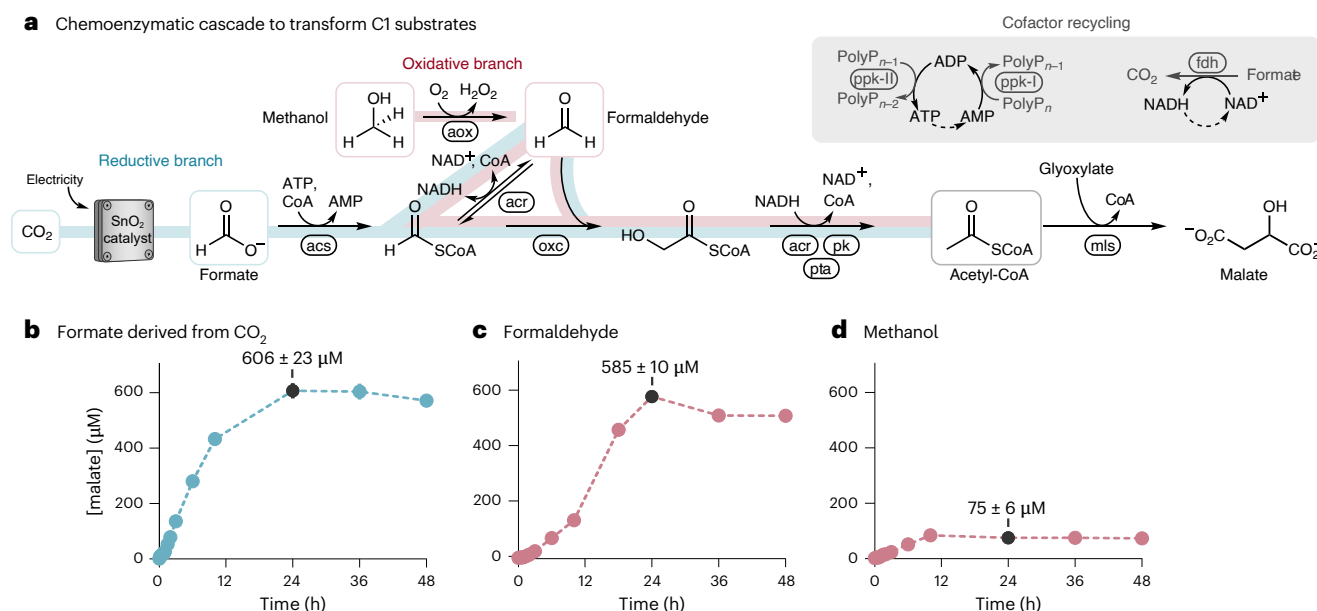
Fig. 5 | Chemoenzymatic conversion of C1 substrates into acetyl-CoA. a , The combined chemoenzymatic cascade enables the assimilation of C1 substrates (formate, \text{CO}_2 , formaldehyde and methanol) into acetyl-CoA. Malate synthase (mls) is added to convert acetyl-CoA into malate. Formate and \text{CO}_2 can be assimilated through the reductive branch of ReForm, while formaldehyde and methanol can be assimilated through the oxidative branch. b–d , Time course of malate synthesis with formate derived from the electrochemical reduction
